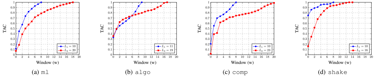
Fig. 6: TAC with different windows w . The TAC curves all exhibit sharp increases initially, indicating many links form around the time they are predicted to. The links at higher w , on the other hand, indicate potential for recommending early link formation and future reconnection.
